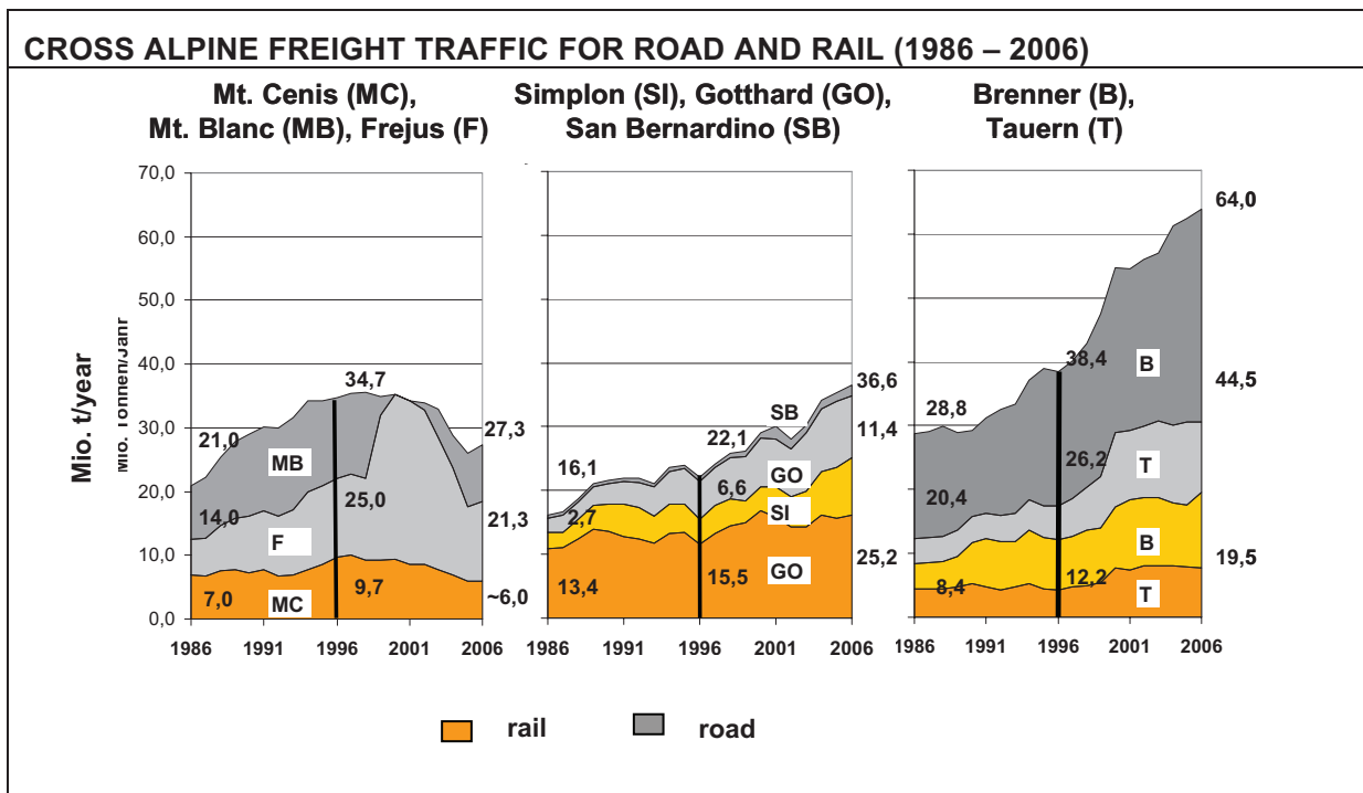
Figure 5 Freight development along the Mt. Cenis, Fréjus, Mont-Blanc, Simplon, Gotthard, San Bernardino, Brenner and Tauern for road and rail. For this evaluation the eight main corridors of the Alpine arc were taken into consideration in order to show the shifts between the corridors. Source: BAV Alpinfo 1986 – 2006
