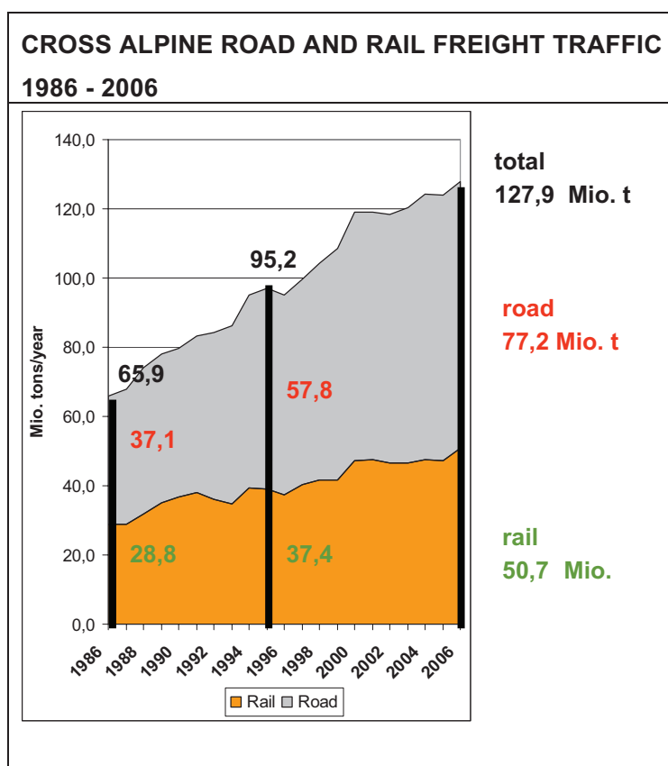
Figure 1 Freight development 1986-2006 across Mt. Cenis, Fréjus, Mont-Blanc, Simplon, Gotthard, San Bernardino, Brenner and Tauern for road and rail transport. Source: BAV Alpinfo 1986 – 2006
