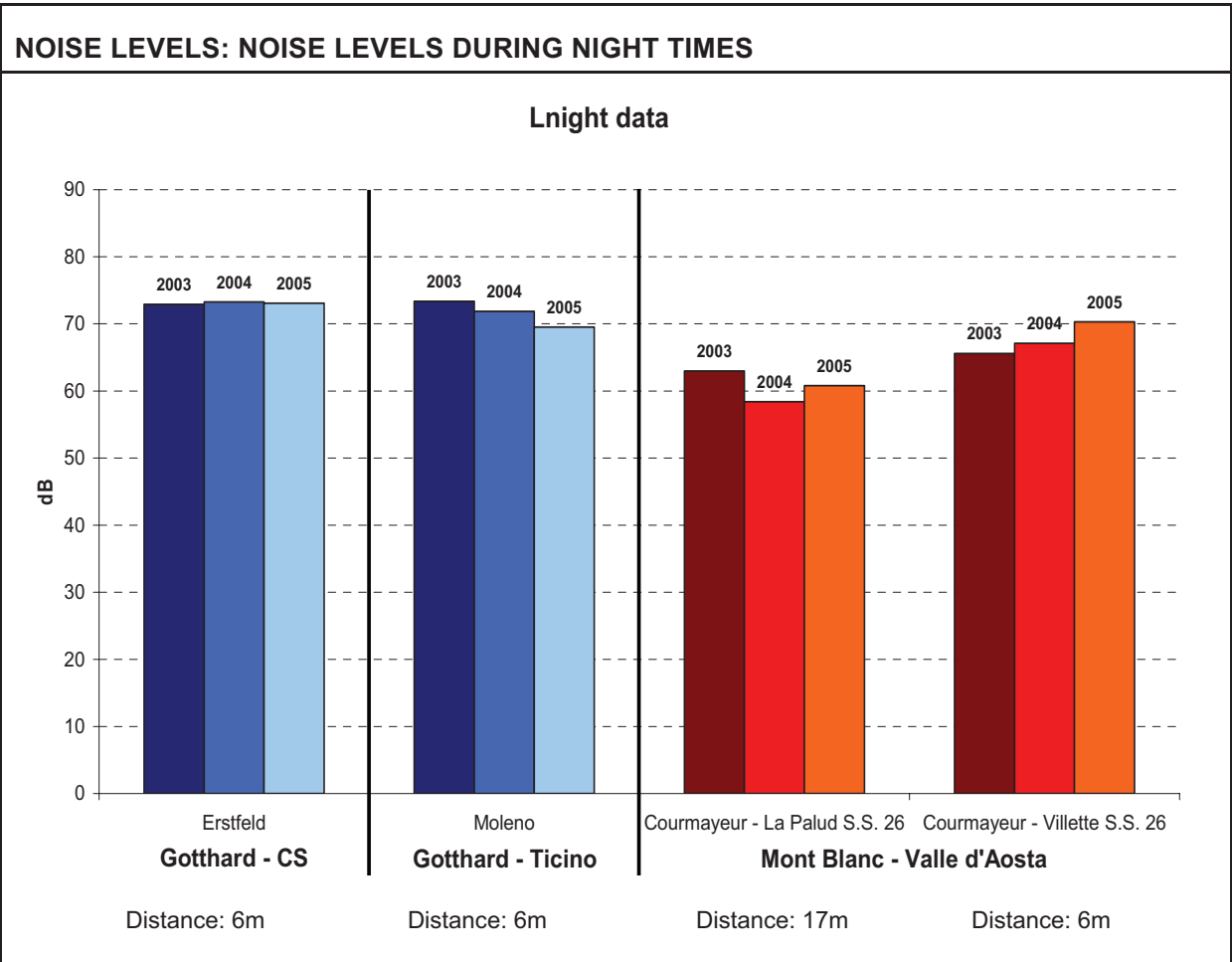
Figure 19 The distance of the microphone from the road is indicated for each station (note that the increase of the distance from 6 m to 17 m may result in a decrease of the noise levels of 4 dB to 5 dB). Source: MONITRAF 2007
