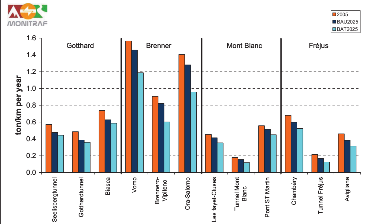
Figure 21 HGV emissions of PM10 for the year 2005 and 2025 calculated for the BAU and BAT scenario. Source: MONITRAF 2007
