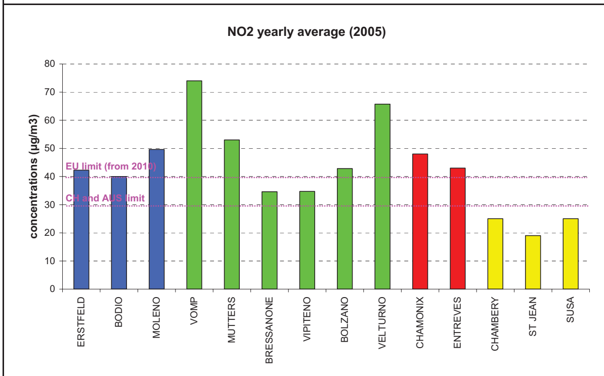
Figure 17 Note that for Tyrol for NO 2 in 2005 the limit value (according to the IG-law) was 30 µg/m 3 including a 10 µg/m 3 tolerance margin. The margin will be reduced by 5 µg/m 3 in the year 2010. In 2012 no tolerance margin will be accepted and the limit value of 30 µg/m 3 must be reached. Source: MONITRAF 2007
