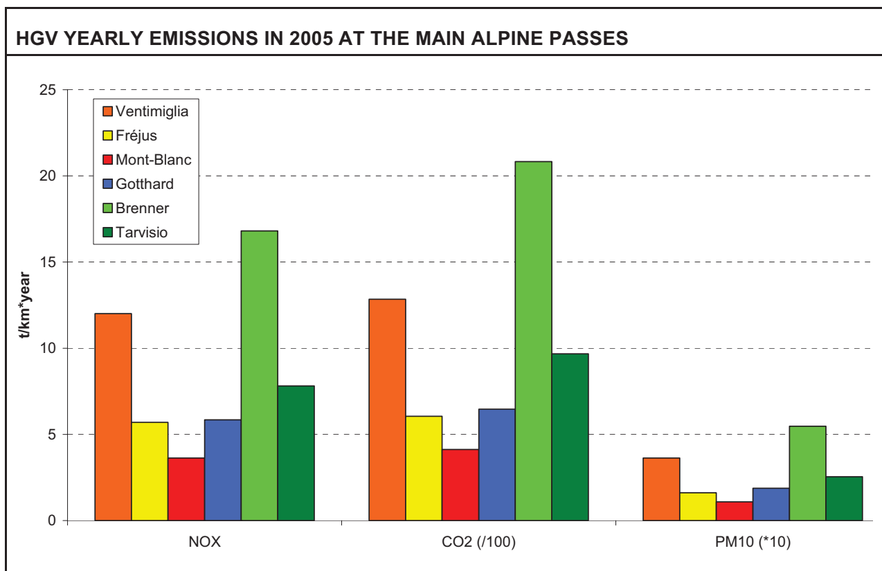
Figure 15 Yearly emission of HGV on the main Alpine corridors evaluated for the year 2005. Source: MONITRAF 2007
