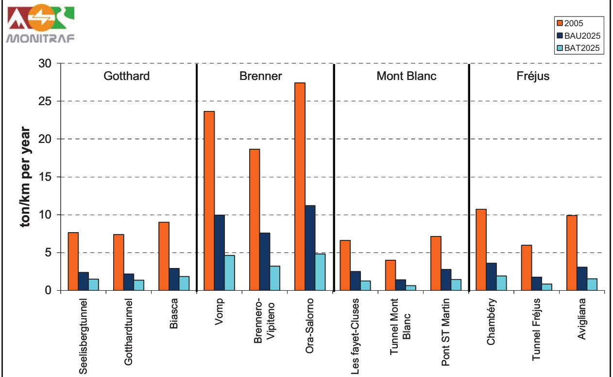
Figure 20 The potential of emission reductions shown in the diagram for 2025 is expected to be reached only under very optimistic conditions. Source: MONITRAF 2007
