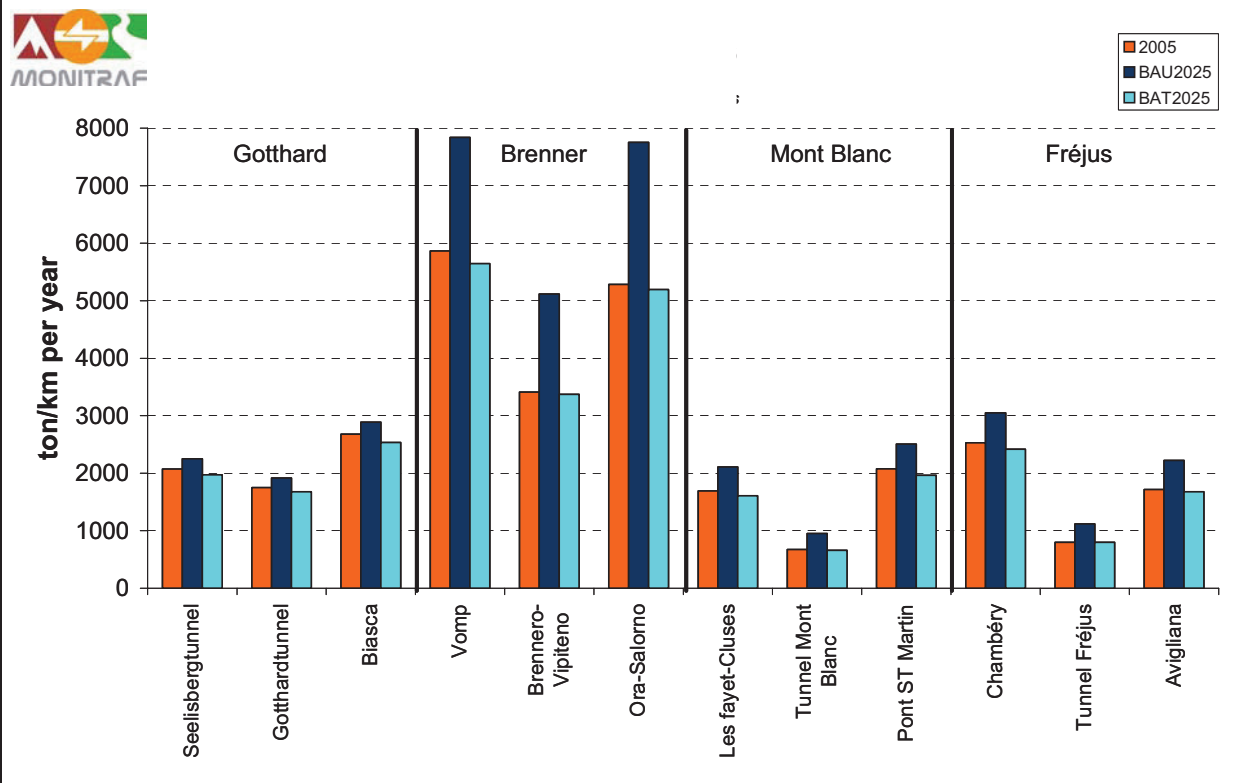
Figure 22 HGV emissions of CO 2 for the year 2005 and 2025 calculated for the BAU and BAT scenario. Source: MONITRAF 2007
