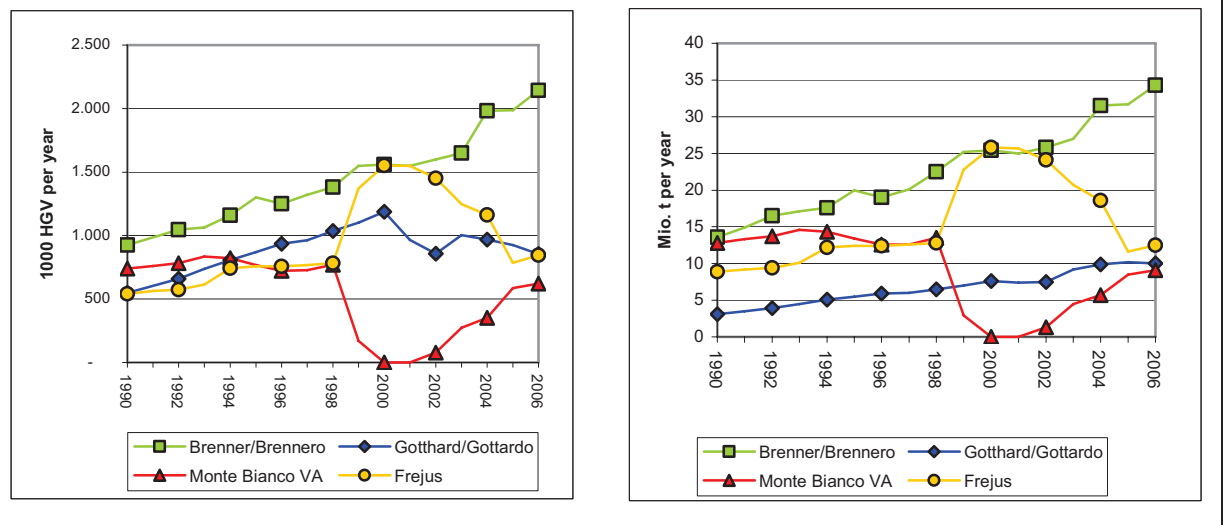
Figure 6 Development of the road freight traffic in 1000 HGV/year (left diagram) and in Mio. tons per year (right diagram) of road freight transport. Source: BAV Alpinfo 1990 – 2006
